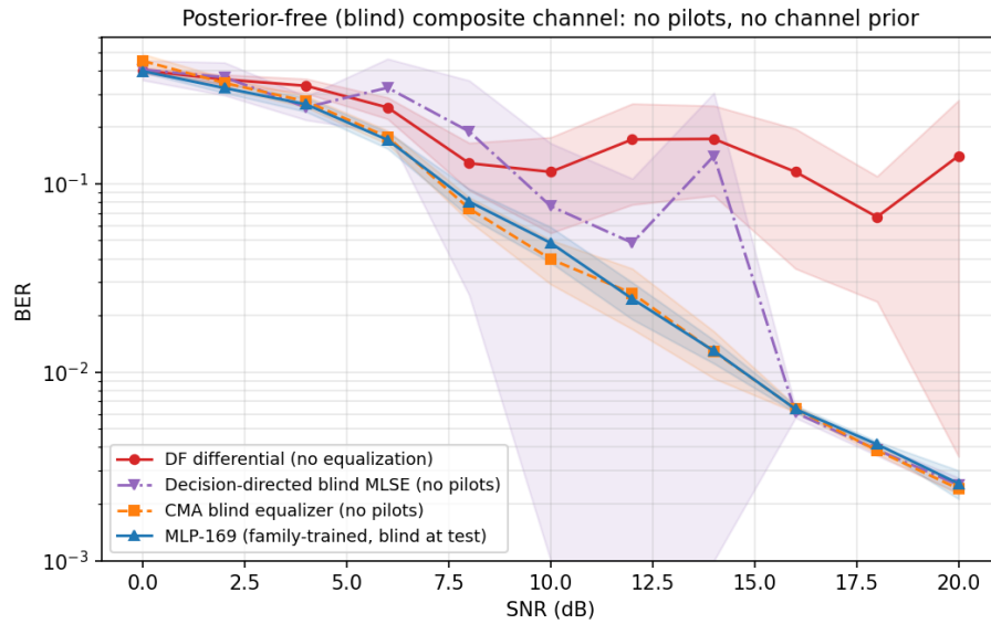
Figure 7.5: Posterior-free composite channel (no pilots, no channel prior, fresh realization per block; mean over 5 trials, 40,000 bits/point). CMA (blind classical) and the family-trained MLP converge together; decision-directed blind MLSE is unstable (non-monotonic, wide CI) because it bootstraps the channel from its own decisions; plain differential detection floors. Without a posterior, learning matches, not beats, the best blind classical equalizer, but does so with one-shot, stable inference and no online adaptation.
