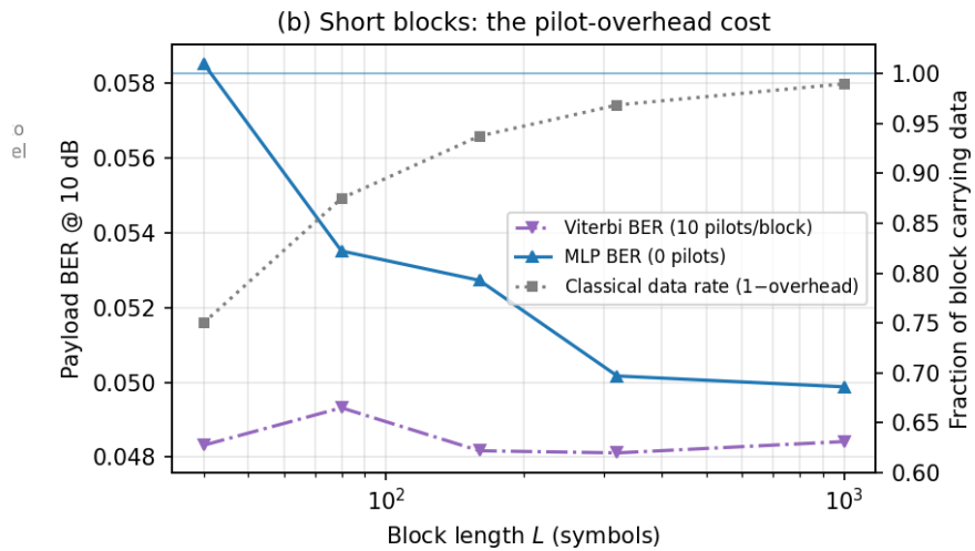
Figure 7.7: Block-length sweep with 10 pilots per block (mean over 6 trials, 40,000 bits/point). Payload BER remains similar across methods, but the effective pilot overhead of the classical approach increases rapidly as the block length decreases, growing from approximately 1% at L = 1000 to 25% at L = 40 . The pilot-free MLP incurs no such overhead and therefore becomes increasingly attractive for short packets.
