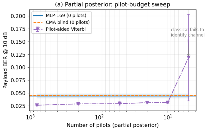
Figure 7.6: Pilot-budget sweep at 10 dB (mean over 6 trials, 40,000 bits/point). Pilot-aided Viterbi outperforms the pilot-free MLP down to approximately 10 pilots per block, but collapses at 5 pilots when the least-squares channel estimate becomes too noisy to construct a reliable trellis ( 0.119 \pm 0.084 ). In contrast, the MLP remains essentially unchanged because it operates with an amortized posterior and requires no pilots.
