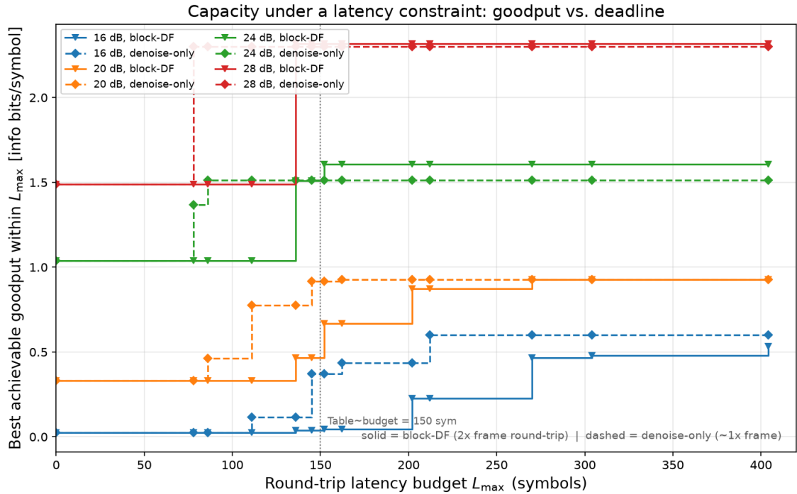
Figure 5.3: Best achievable goodput as a function of the round-trip latency budget L_{\max} , at the four SNRs where the two relay strategies differ (16, 20, 24, 28 dB). Each curve is a step function: goodput jumps each time L_{\max} crosses an MCS's round-trip latency. The denoise-only relay's steps (dashed) occur at roughly half the L_{\max} of the block-DF relay's (solid) for a comparable rate, since block-DF pays the frame cost twice.
