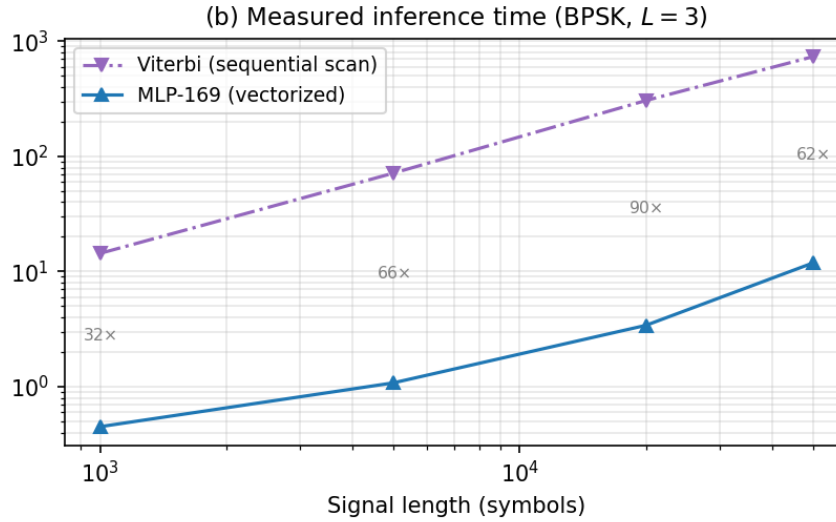
Figure 6.8: Measured inference time for BPSK with L = 3 : the MLP is 30–90 \times faster as a vectorized matmul versus Viterbi’s interpreted sequential trellis scan.
