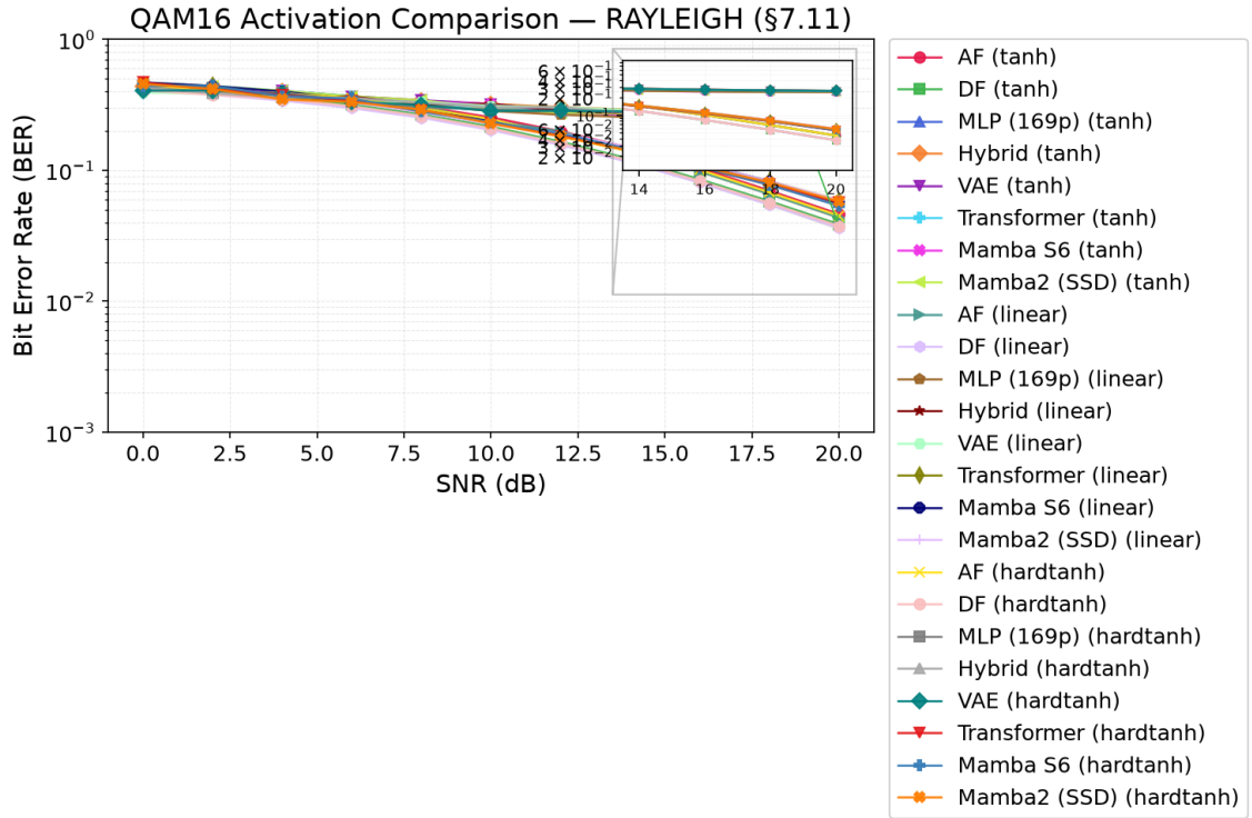
Figure 6.3: 16-QAM activation study on the canonical Rayleigh channel. Each relay appears three times, once per output activation — tanh (the BPSK-trained baseline), linear, and hardtanh clipped to 3/\sqrt{10} — distinguished by colour and marker. The separation is by model family rather than by activation: the three sequence models drop by roughly half when their output is bounded, while the feedforward relays are essentially unchanged (Table 6.2).
