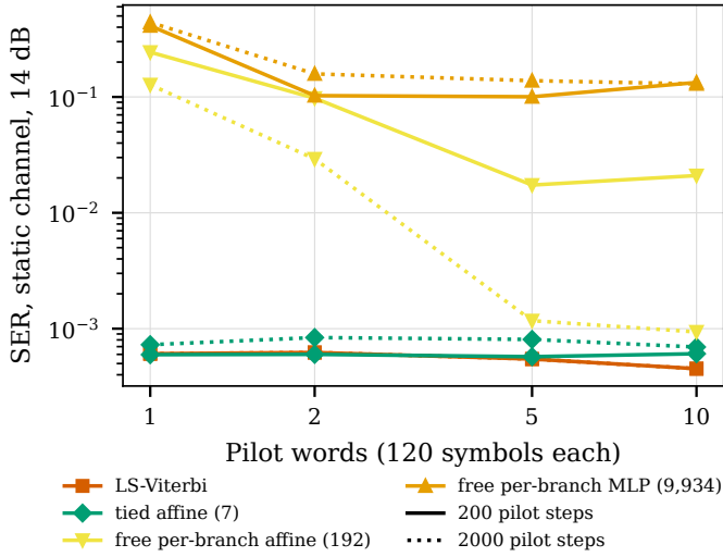
Fig. 14. QPSK on a static channel at 14 dB: SER vs. pilot length with 200 (solid) or 2,000 (dotted) pilot training steps. Parentheses: trainable parameters.
