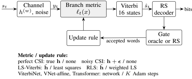
Fig. 2. Common receiver structure. Only the shaded branch-metric block and its update rule differ between receivers; every adaptive receiver adapts on the same pilots and accepted words.
