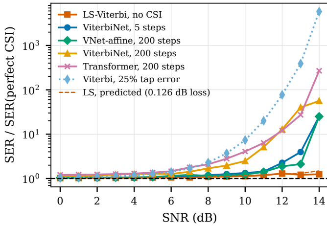
Fig. 2. SER relative to the perfect-CSI Viterbi detector. Dashed red: LS-Viterbi predicted by (2). At 14 dB the K = 5 , VNet-affine, and LS points rest on 4 error events each.
