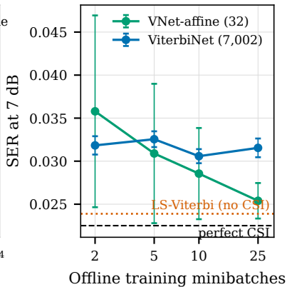
(b) offline budget, 200 online steps
