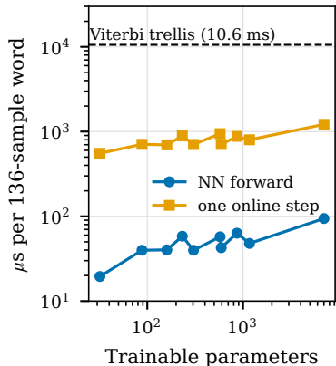
(c) latency, one CPU thread
