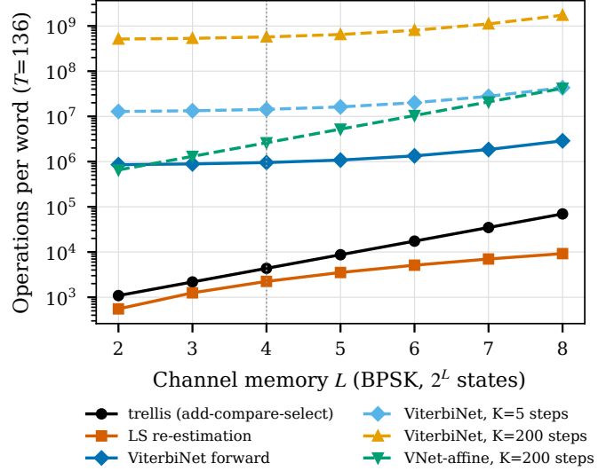
Fig. 3. Operations per 136-sample word vs. channel memory (BPSK). Network costs scale the 1 \rightarrow 100 \rightarrow 58 \rightarrow 2^L ViterbiNet and the 2 \cdot 2^L -parameter affine metric; adaptation counts forward and backward passes. Dotted line: L = 4 used in this paper.
