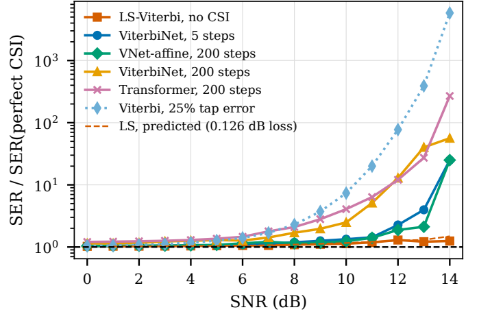
Fig. 2. SER relative to the perfect-CSI Viterbi detector. Dashed red: LS-Viterbi predicted by (2). At 14 dB the K = 5 , VNet-affine, and LS points rest on 4 bit errors each, clustered in one or two repetitions.
