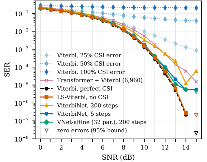
Fig. 4. BPSK SER vs. SNR. LS-Viterbi receives the same pilots and accepted decisions as the learned receivers; noisy-CSI curves perturb the taps by a fixed fraction. Hollow triangles: no errors observed (95% upper bound).
