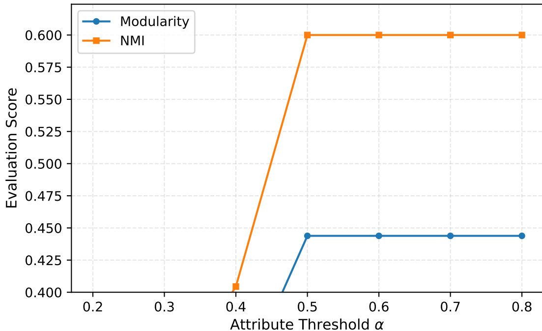
Effect of Attribute Threshold \alpha on Detection Performance
