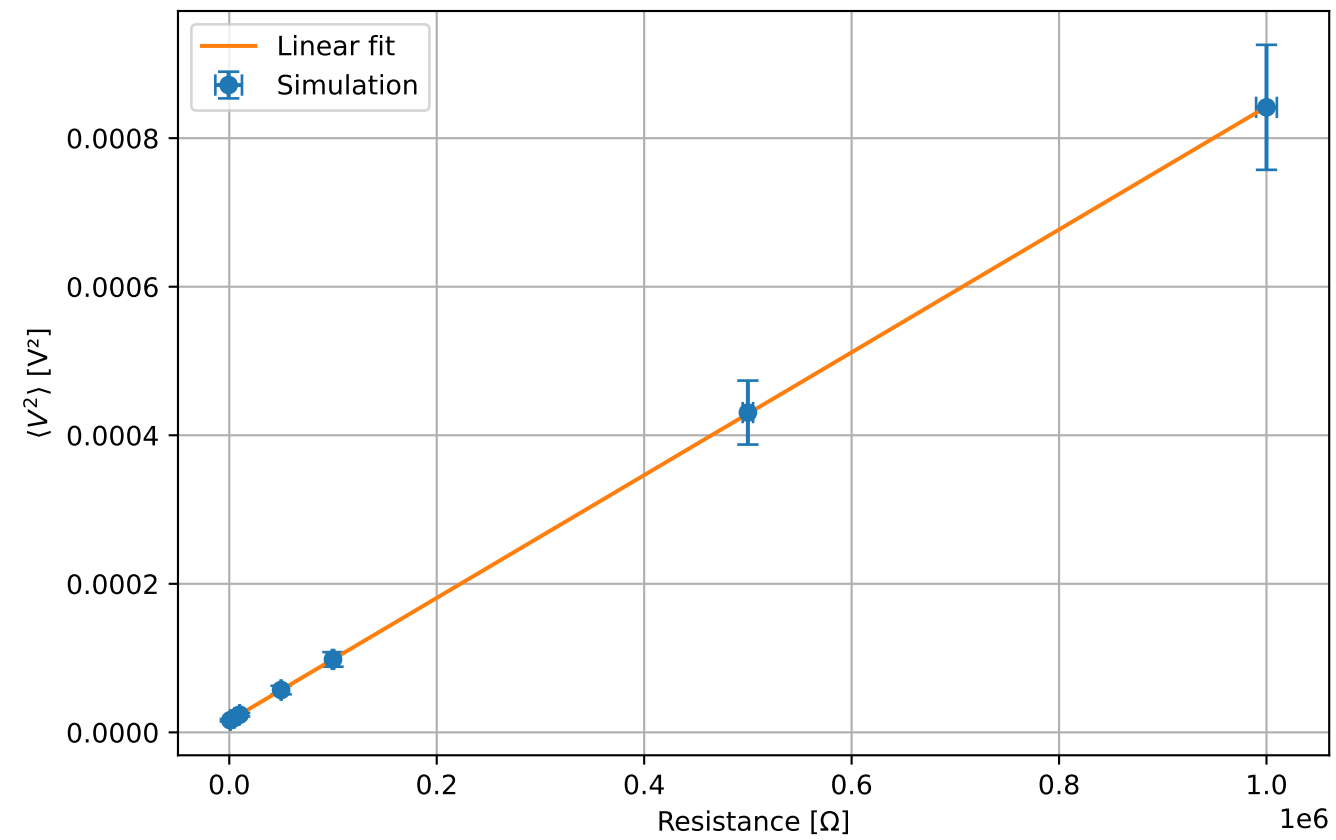
\langle V^2 \rangle vs Resistance
