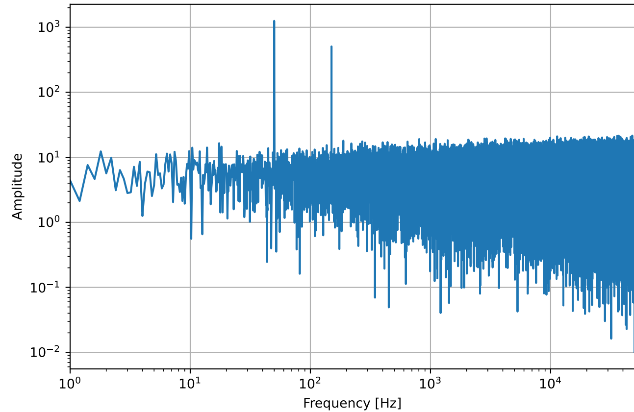
Raw FFT Spectrum (100 k \Omega )
