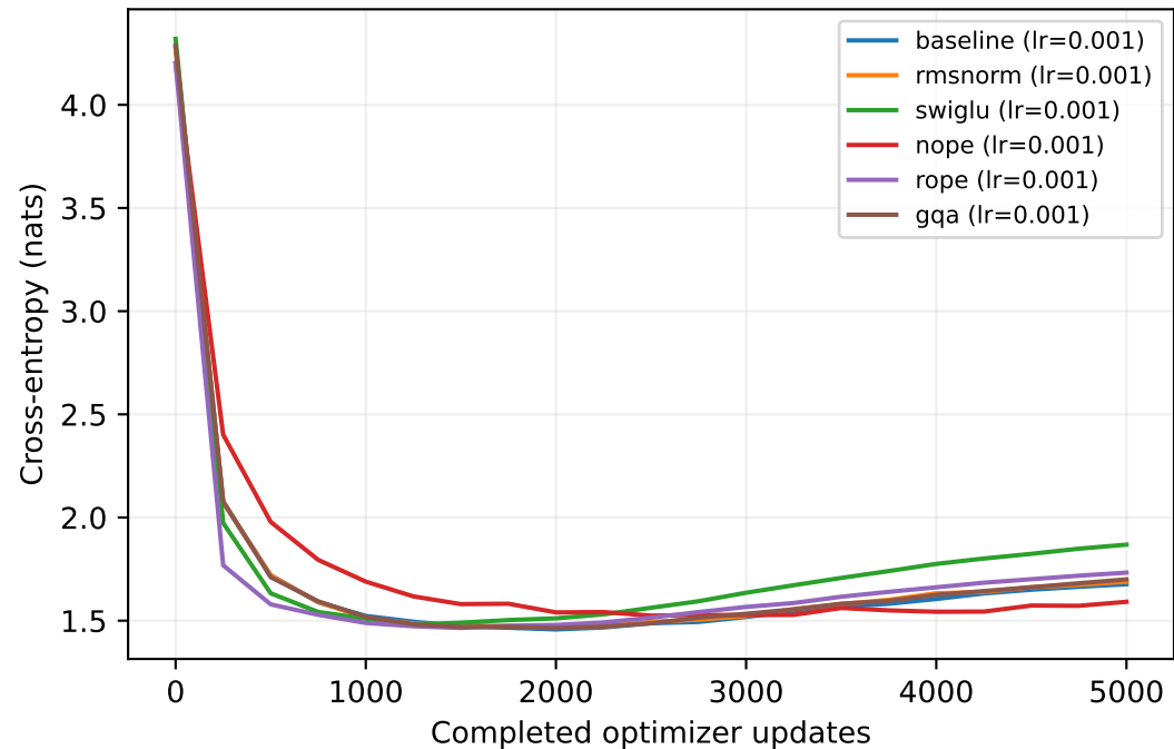
Validation loss
