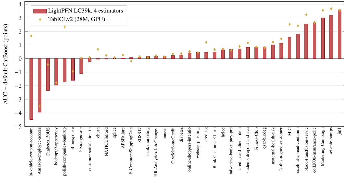
Figure 9. TabArena full protocol: AUC difference to default CatBoost on each of the 38 classification tasks, in points, for LightPFN LC39k with four estimators (bars, sorted) and TabICLv2 (diamonds). Ranks use the log loss for the 8 multiclass tasks, so the share of tasks won in Table 10 (76%) differs slightly from the 28 of 38 tasks with higher AUC here.
