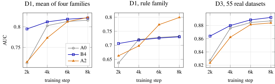
Figure 7. AUC of the EMA checkpoints after 2,000 to 8,000 steps of the ablations. B4 leads early and keeps about half a point at the end; A2 (graph v4 and rule tasks) starts slower and is still rising on the rule family when the ablation stops.
