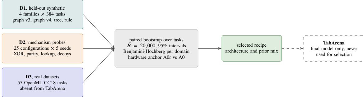
Figure 5. Selection protocol. Design decisions are taken on D1, D2 and D3 with paired statistics (the long-context stage also on learning curves of the largest D3 datasets, Section 9); TabArena is reserved for the final models.
