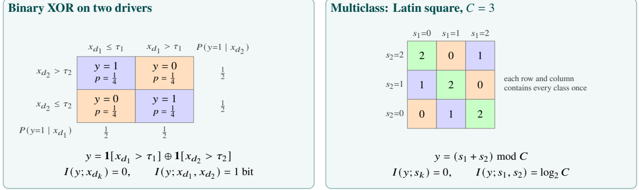
Figure 3. Interaction-only rule tasks. Left: binary XOR on two drivers whose source thresholds split balanced factorial cells, so each driver alone predicts the label at chance. Right: for C classes, symbols of two drivers are summed modulo C , a Latin square in which every row and column contains each class once.
