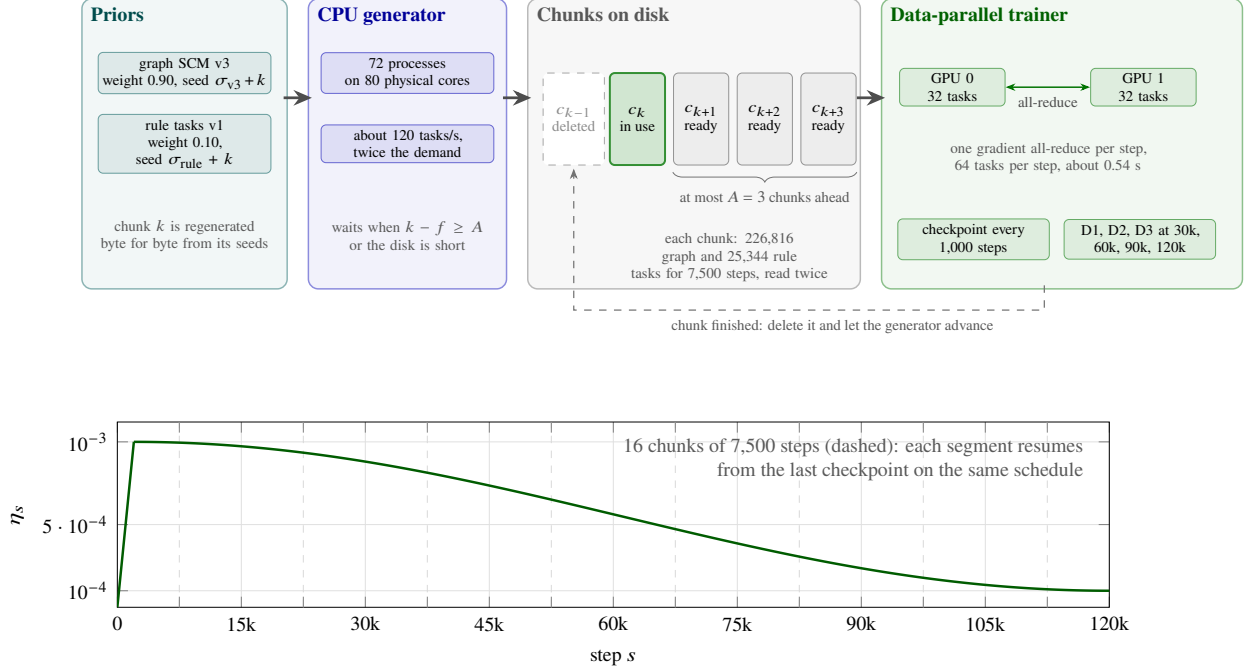
Figure 4. Training system of the final run. Top: CPU processes generate chunks of fresh tasks from the priors, at most A = 3 chunks ahead of the trainer; two GPUs train on the current chunk with one gradient all-reduce per step, and every finished chunk is deleted. Bottom: the learning rate over the 120,000 steps; the sixteen segments, one per chunk, resume from checkpoints and follow one warmup and cosine schedule.
