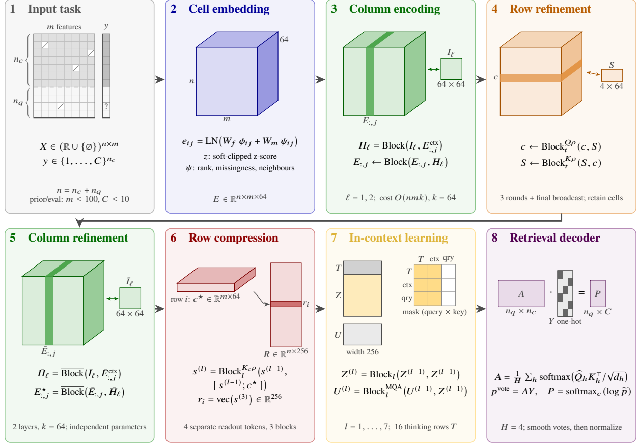
Figure 1. B4 from the input table through seven operators. Both column stages gather from labelled context cells and broadcast to context and query cells. Row refinement exchanges information through temporary summaries while retaining the cells; row compression uses a separate set of summaries. The second column stage is an explicit step between refinement and compression. Tensor shapes, attention directions and the context/query mask are shown for one task.
