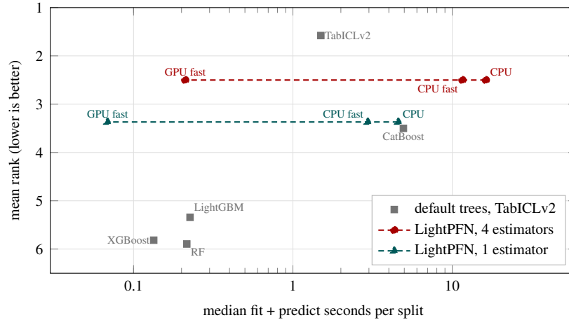
Figure 10. TabArena full protocol: mean rank against the median fit plus predict time per split (log scale). Each LightPFN line joins the initial CPU evaluation, the CPU rerun with the new inference defaults and the GPU rerun, which have the same predictions up to rounding and the same rank. Hardware as in Table 12; the different hosts and concurrency settings prevent a controlled comparison across models.
