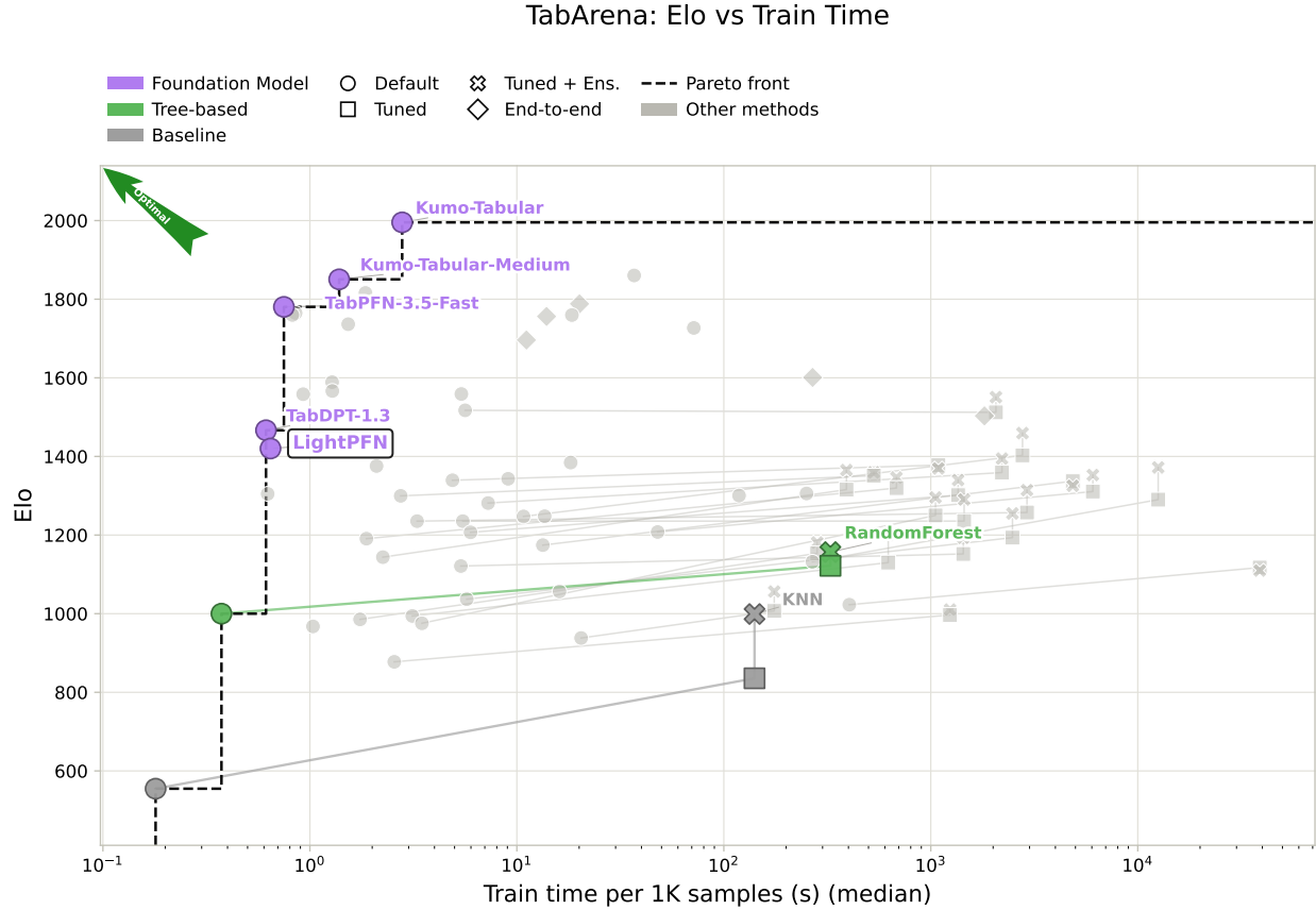
Figure 11. Official TabArena-Lite classification: Elo against median fit time per 1,000 rows, from the leaderboard snapshot. LightPFN is highlighted in the foundation-model color. Hardware differs across methods.
