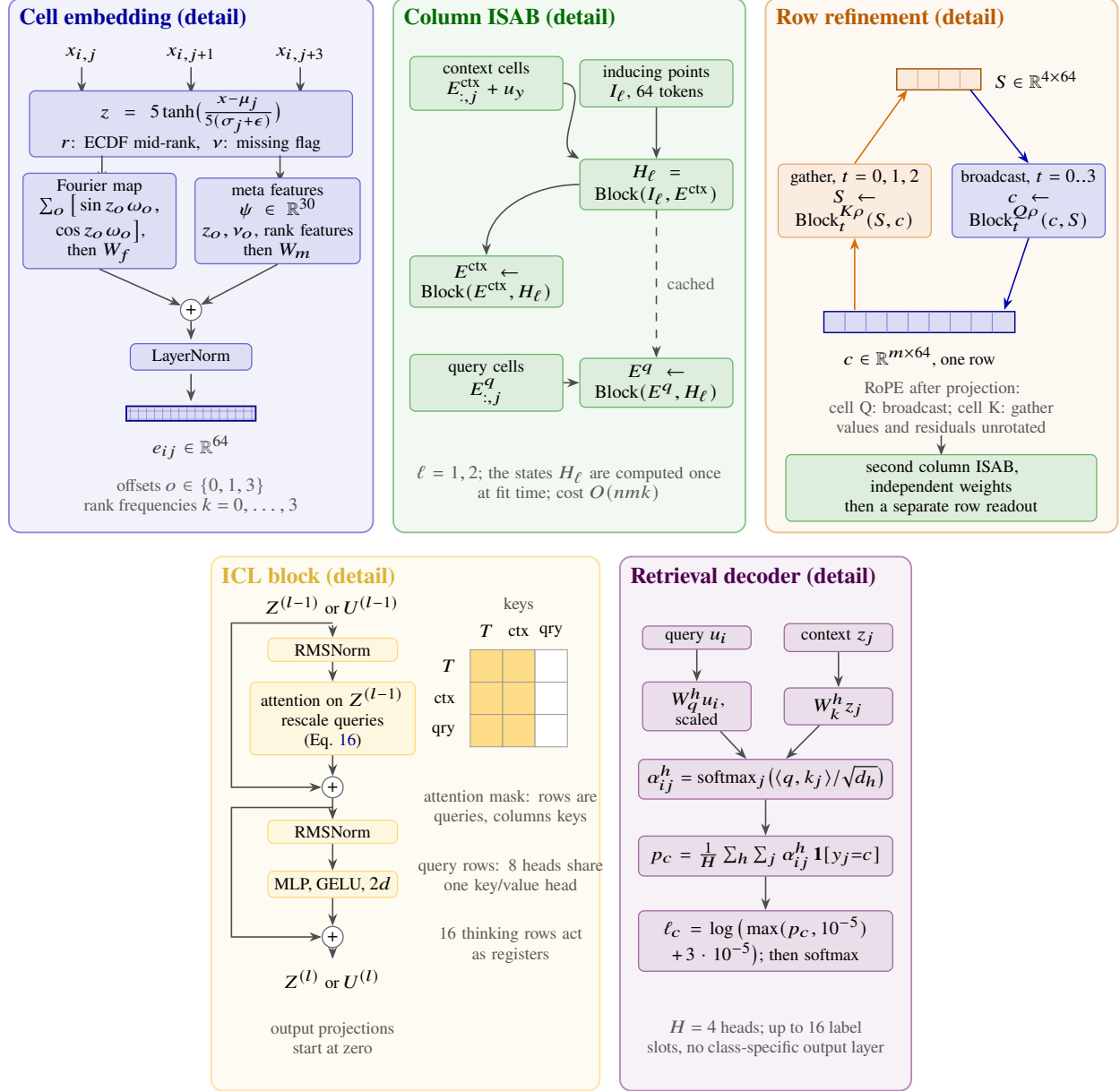
Figure 2. Cell embedding, column ISAB, row refinement, an ICL block and label retrieval. The dashed column arrow denotes cached memory. Rotary positions act on projected cell queries in broadcast and on projected cell keys in gather and pooling. Cell values and residual states are unrotated. The column pattern is used twice with independent parameters.
