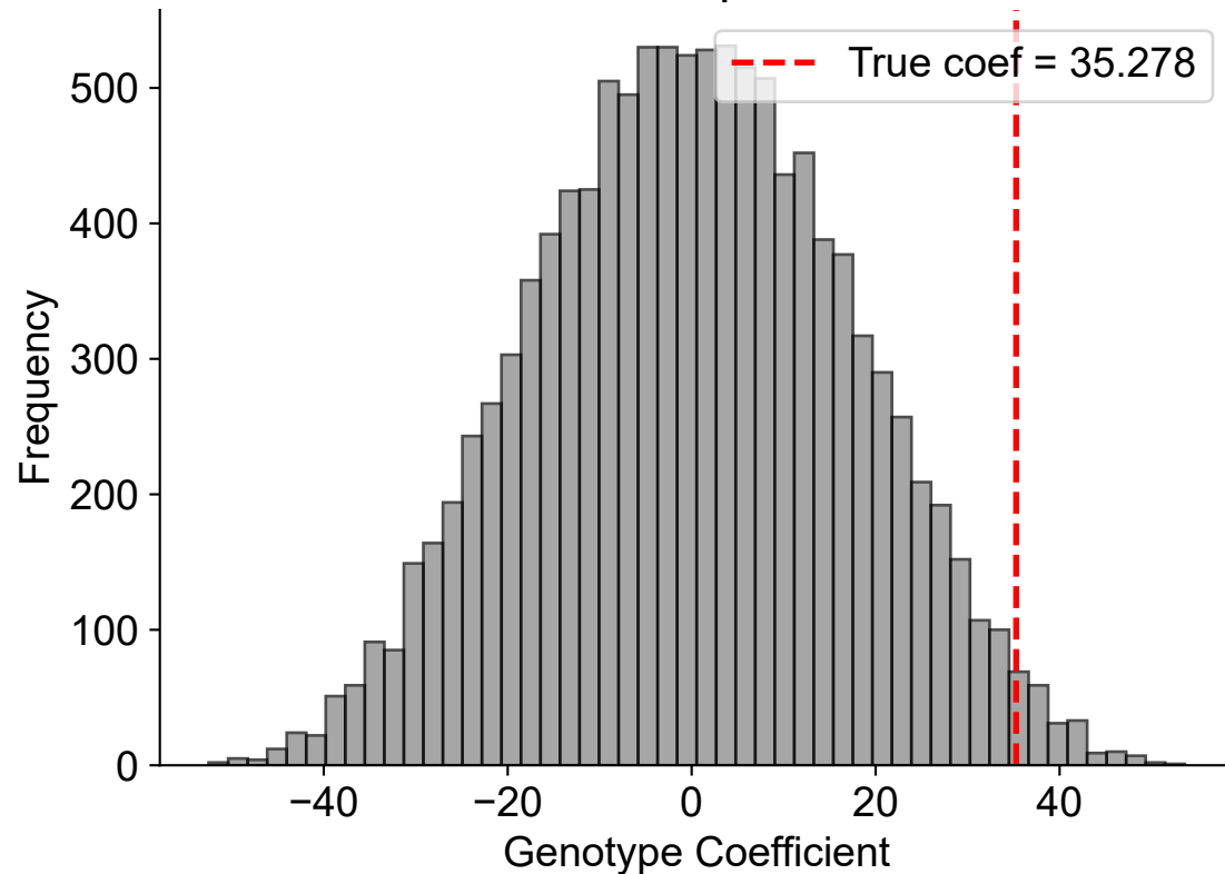
cov_rank Permutation p = 0.0331
