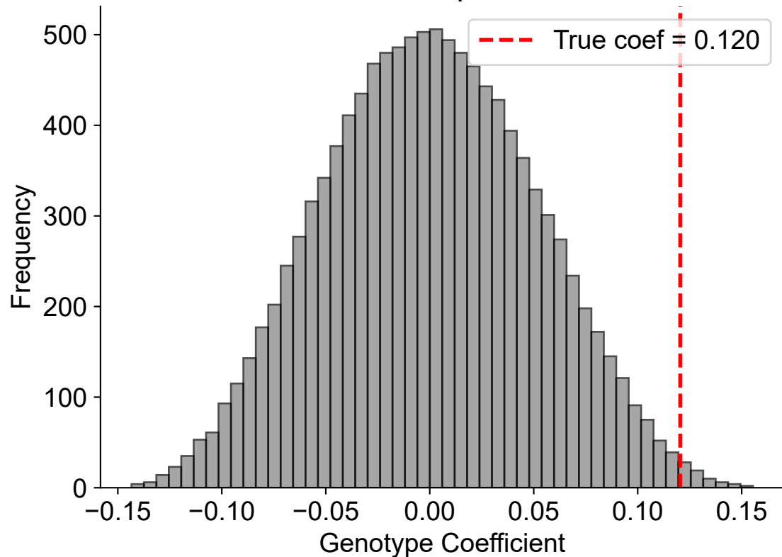
cov Permutation p = 0.0094
