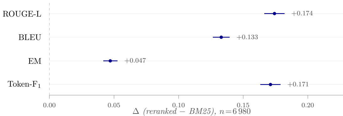
Figure 7. Headline paired-bootstrap forest plot (Table 12). Dots: per-query mean \Delta (reranked – BM25); bars: 95 % percentile interval, 10 000 resamples, seed 42. Dashed line at zero: all four intervals lie strictly above it, two-sided bootstrap p < 0.001 throughout.
