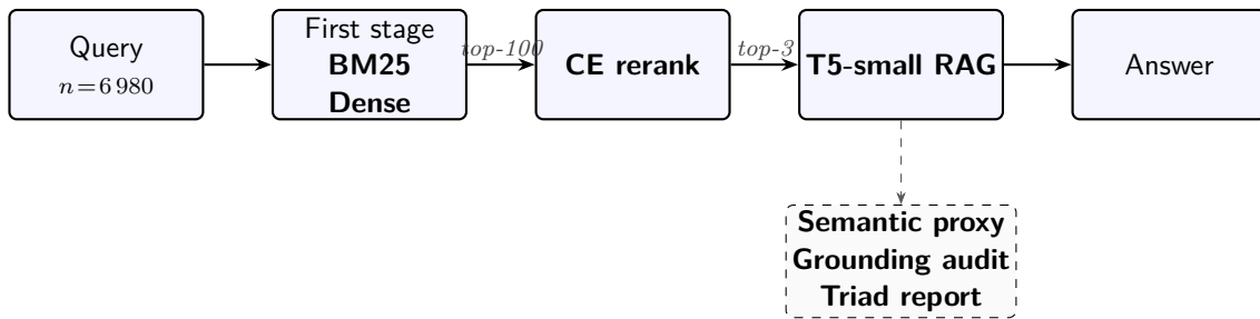
Figure 5. End-to-end pipeline. Solid boxes are the four modelling stages of Section 4; the dashed box is the post-hoc evaluation layer (Sections 5.9 and 5.10), plus the current triad diagnostic interface, which consumes the already-on-disk paired generation predictions and does not re-run any modelling stage. BM25 and dense retrieval are interchangeable first stages feeding into the same downstream pipeline; the paired generation comparison of Section 5.7 switches between them.
