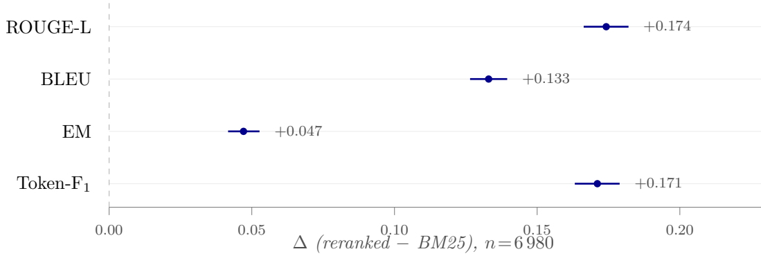
Figure 7. Headline paired-bootstrap forest plot (Table 9). Dots: per-query mean \Delta (reranked – BM25); bars: 95 % percentile interval, 10 000 resamples, seed 42. Dashed line at zero: all four intervals lie strictly above it, two-sided bootstrap p < 0.001 throughout.
