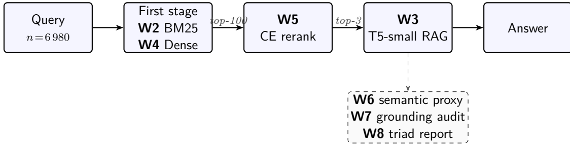
Figure 5. End-to-end pipeline. Solid boxes are the four modelling stages of Section 4; the dashed box is the post-hoc evaluation layer (Sections 5.8 and 5.9), plus the current triad diagnostic interface, which consumes the already-on-disk W3 paired predictions and does not re-run any modelling stage. W2 and W4 are interchangeable first stages feeding into the same downstream pipeline; the W3 paired comparison of Section 5.6 switches between them.
