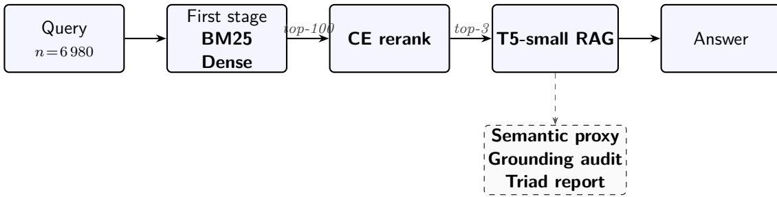
Figure 5. End-to-end pipeline. Solid boxes are the four modelling stages of Section 4; the dashed box is the post-hoc evaluation layer (Sections 5.13 and 5.14), plus the current triad diagnostic interface, which consumes the already-on-disk paired generation predictions and does not re-run any modelling stage. BM25 and dense retrieval are interchangeable first stages feeding into the same downstream pipeline; the paired generation comparison of Section 5.11 switches between them.
