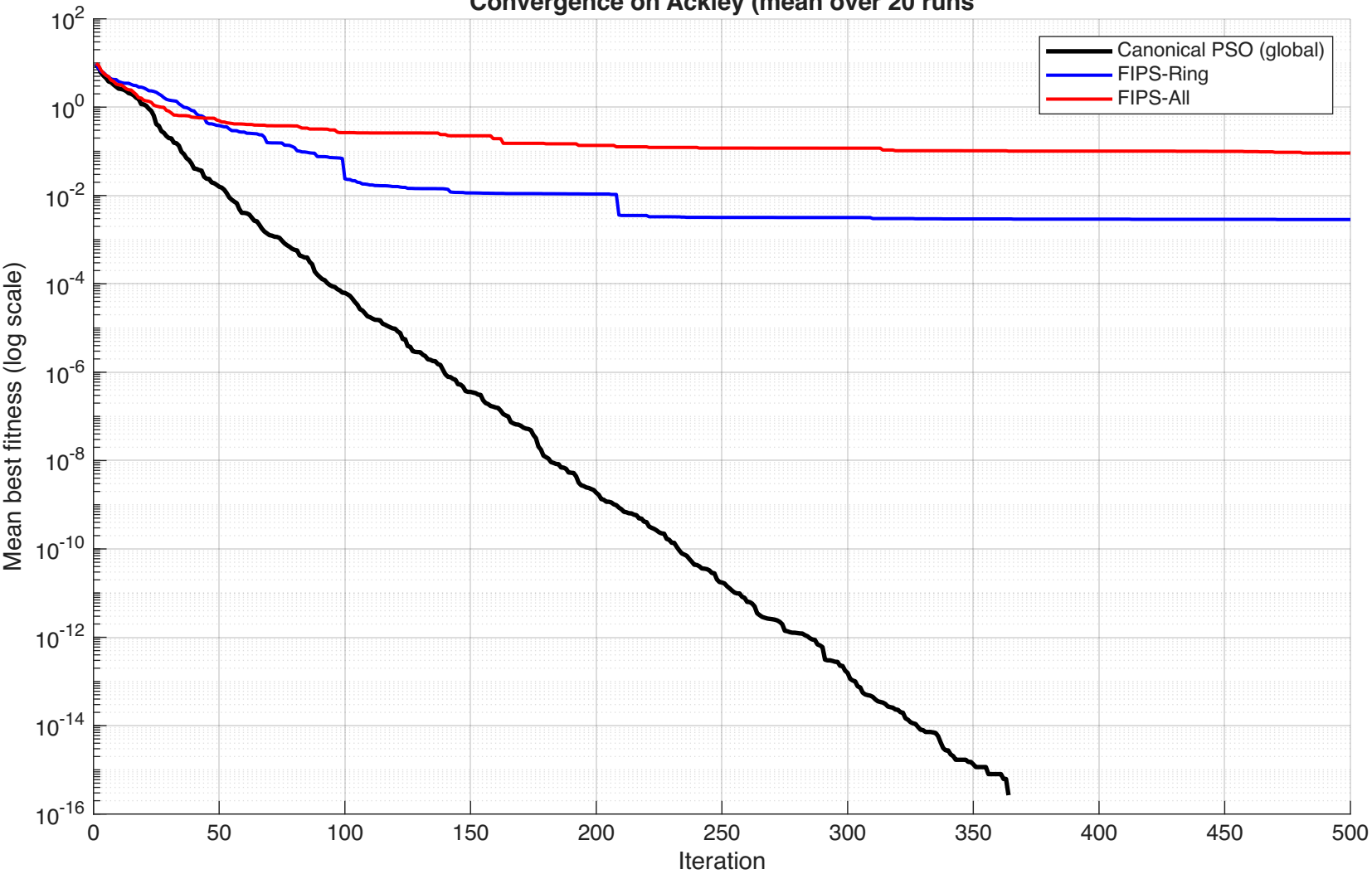
Convergence on Ackley (mean over 20 runs)
