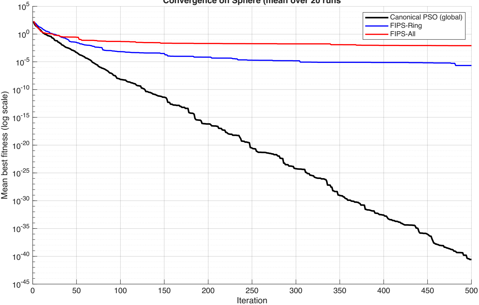
Convergence on Sphere (mean over 20 runs)
