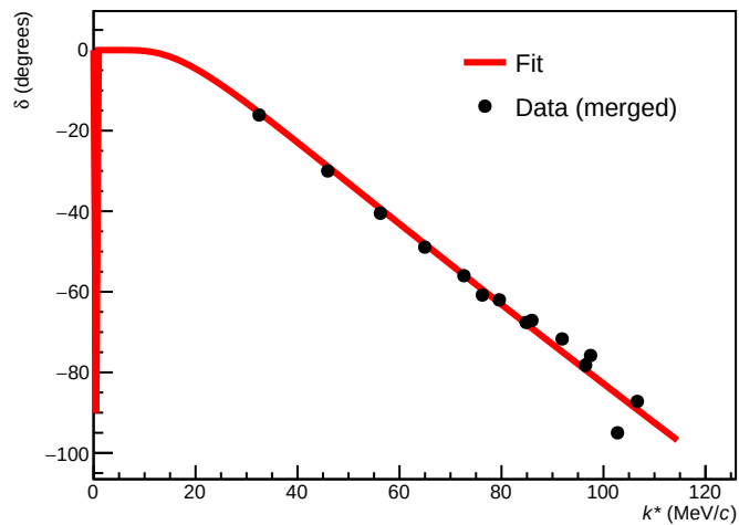
L=0, S=1 ( ^3S_1 )
