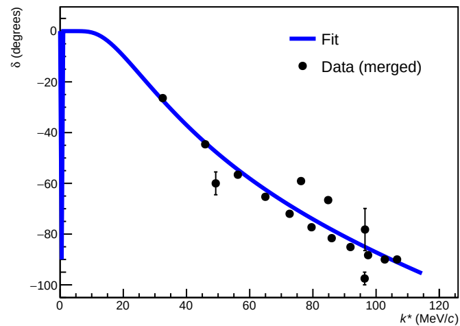
L=0, S=0 ( ^1S_0 )
