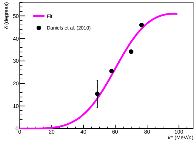
L=1, S=1 (triplet, p-wave)
