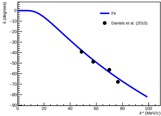
L=1, S=0 (singlet, p-wave)
