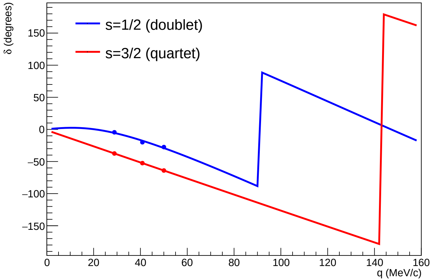
p-d Phase Shifts: Fitted Theory vs Target Values
