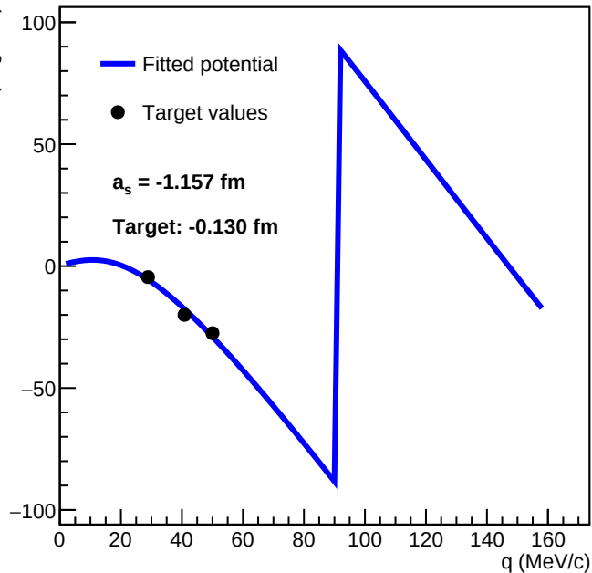
s=1/2 (doublet)
