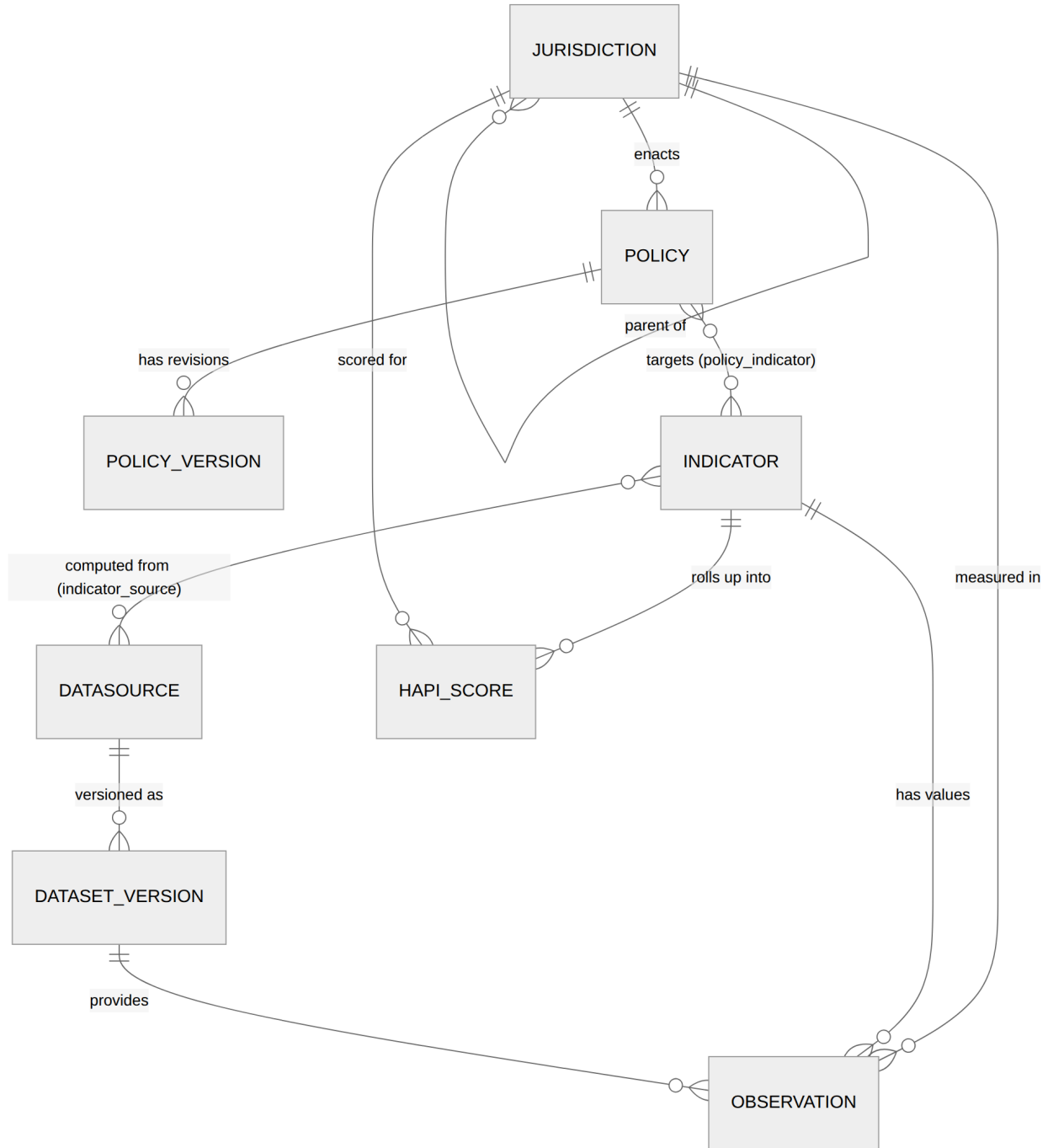
Figure 4. Entity-relationship model. Every value resolves along the lineage chain
