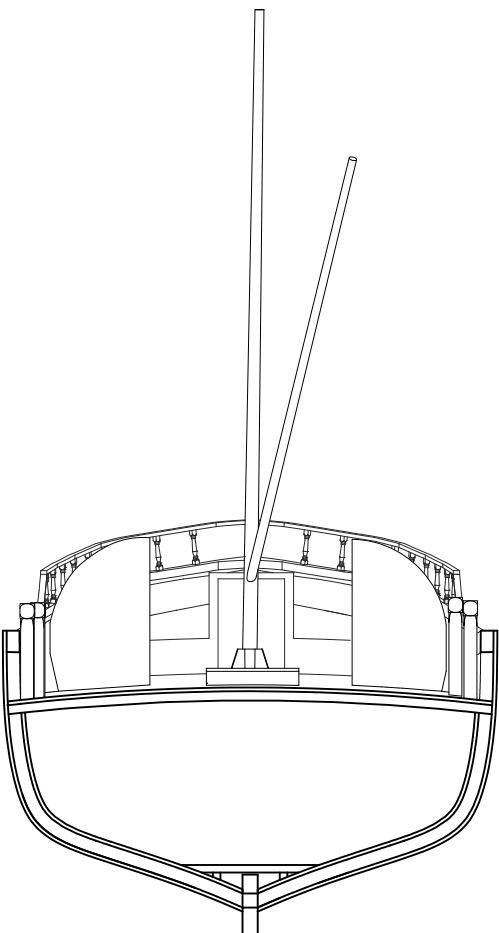
Cross Section (Bow)
