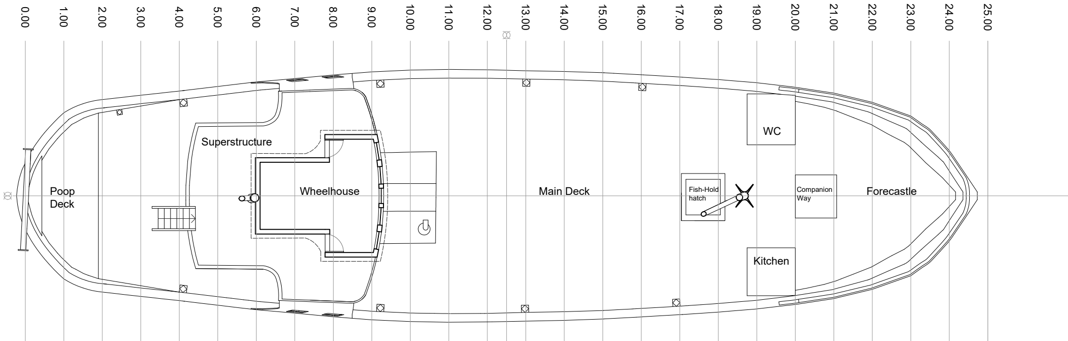
Plan View of Upper Deck - Level 6.60m
