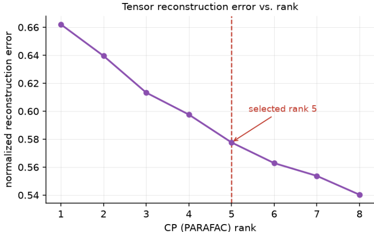
Figure 2: Tensor reconstruction error vs. CP (PARAFAC) rank. Normalised Frobenius reconstruction error over the observed (unmasked) entries of the 71 \times 1650 \times 8 \times 8 communication tensor, for non-negative decompositions of rank 1–8 (single seed, random_state=0 , matching the in-fold projector). The error decreases smoothly with diminishing returns rather than at a sharp elbow; rank 5 (dashed line) captures roughly two-thirds of the reduction available across this range and was fixed for parsimony and interpretability (see text).
