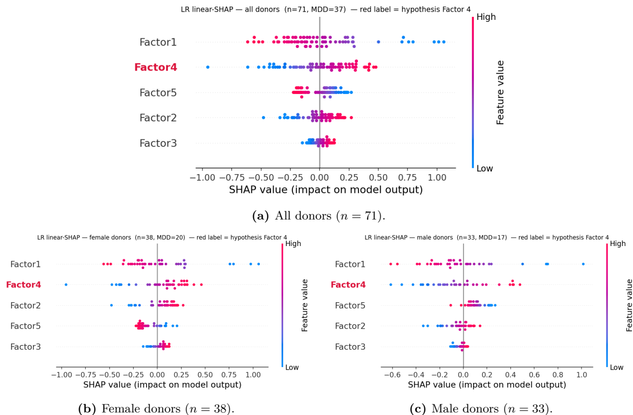
Figure 3: Communication-only logistic-regression SHAP beeswarm (the five factor loadings). Factor 4 (red label) carries among the largest mean|SHAP| and its high values (red) sit on the positive-SHAP side—i.e. a more active microglia → ExN10_L46 program pushes the prediction toward MDD—in both sexes.
