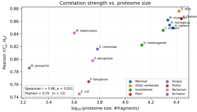
Fig. 10. Strength of the proteome-scale correlation r(f_{cp}^+, H_p) against \log_{10} of proteome size for all thirteen organisms, computed with the identical AlphaFold-DB v6, integer-pLDDT batched pipeline and coloured by clade. The six large proteomes (right) span four clades — mammal, other vertebrate, invertebrate, and plant — yet pack into a tight high- r band; the smaller proteomes (left) fall both lower and more scattered. Colour produces no vertical separation: at matched size the mammals and the large non-mammalian eukaryotes (zebrafish, Arabidopsis , C. elegans ) coincide, so the gradient tracks size , not clade . M. tuberculosis (small, yet r = 0.84 ) is the lone outlier. The per-organism rank correlation of r with \log_{10} N is Spearman 0.86 ( p < 0.001 , n = 13 ).
