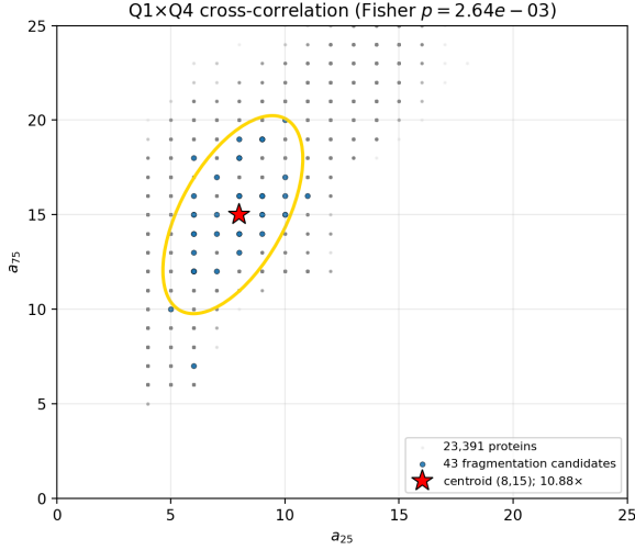
Fig. 6. Q1 \times Q4 cross-correlation. Points show the arity distribution of all 23,391 proteins; the yellow ellipse marks the 95% confidence region of the 43 fragmented proteins (centroid at (8, 15); 10.88-fold enrichment, p = 2.64 \times 10^{-3} ).
