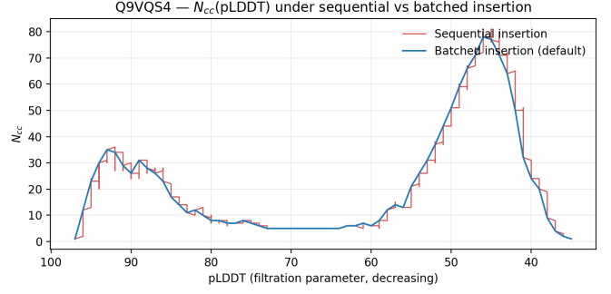
Fig. 7. N_{cc} (pLDDT) curve for the mixed prototype Q9VQS4 under sequential and batched insertion (integer pLDDT in both). The sequential curve carries intra-level transients; the batched curve is piecewise constant within each integer plateau.
