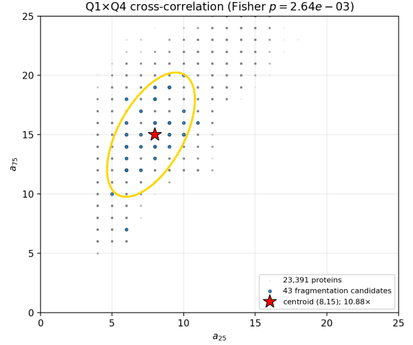
Fig. 6. Q1xQ4 cross-correlation. Points show the arity distribution of all 23,391 proteins; the yellow ellipse marks the 95% confidence region of the 43 fragmented proteins (centroid at (8, 15); 10.88-fold enrichment, p = 2.64 \times 10^{-3} ).
