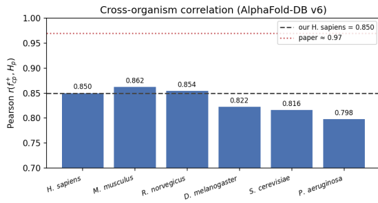
Fig. 10. Proteome-scale Pearson correlation r(f_{cp}^+, H_p) for the six organisms, all computed with the identical AlphaFold-DB v6, integer-pLDDT batched pipeline. The three mammals cluster at our own H. sapiens value (dashed line); the correlation is lower in the three smaller proteomes — the invertebrate D. melanogaster , the yeast, and the bacterium P. aeruginosa (the only out-of-clade point) — yet stays strong throughout ( r \geq 0.80 ). Crucially the fly, whose fragmentation statistics are mammal-like, still falls with the smaller proteomes, so the gradient is not driven by disorder content. The paper’s reported r \approx 0.97 (dotted line) is shown only as an external reference.
