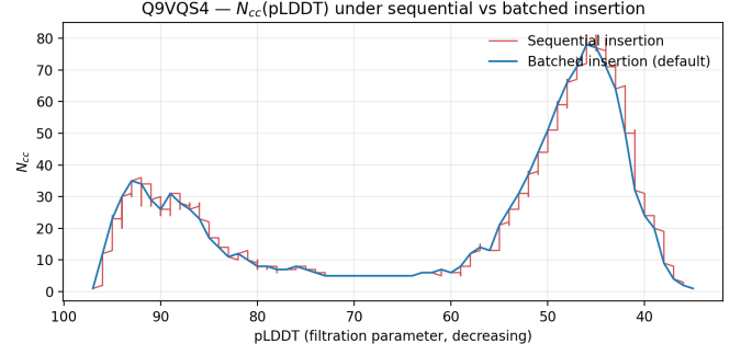
Fig. 7. N_{cc}(\text{pLDDT}) curve for the mixed prototype Q9VQS4 under sequential and batched insertion (integer pLDDT in both). The sequential curve carries intra-level transients; the batched curve is piecewise constant within each integer plateau.
