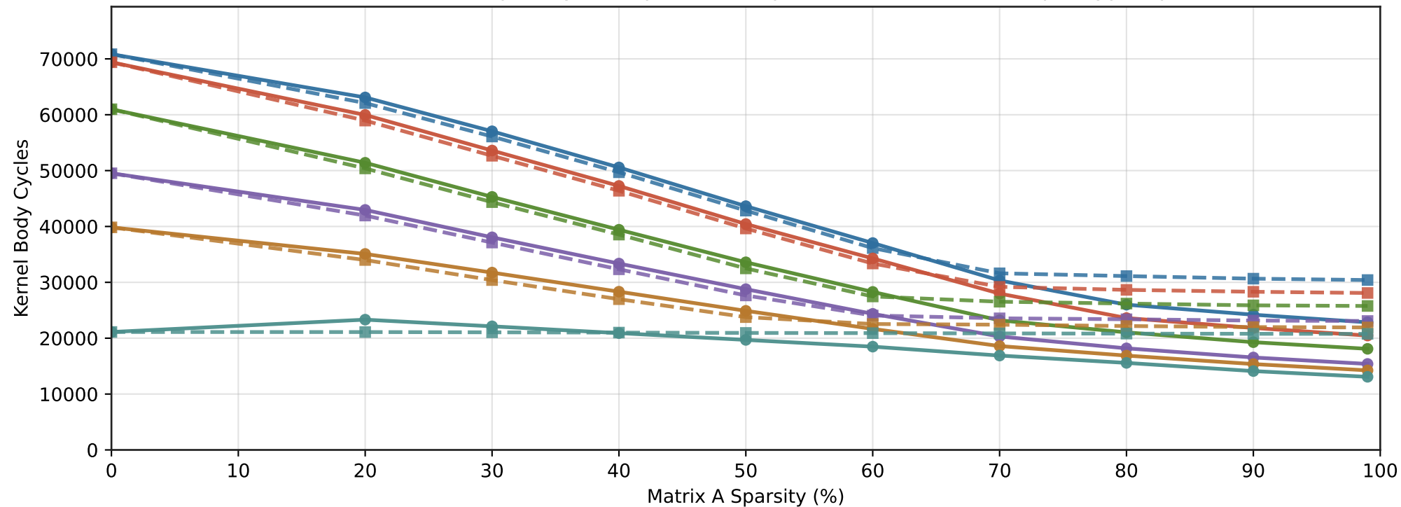
SGEMM TCU OP Sparsity Sweep - Matrix operation: 64x64x512, Input type: fp8
