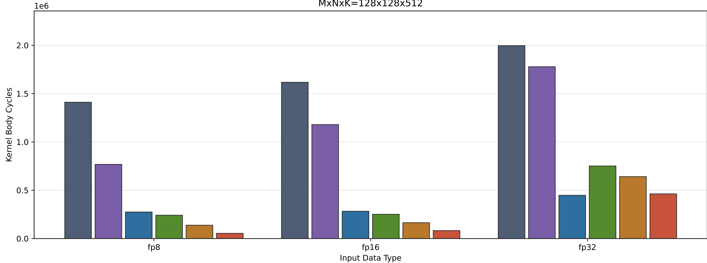
Kernel Body Cycles by Input Data Type MxNxK=128x128x512
