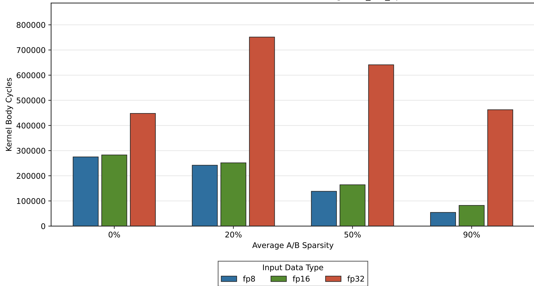
Kernel Body Cycles by OP Sparsity MxNxK=128x128x512, Kernel=sgemm_tcu_op
