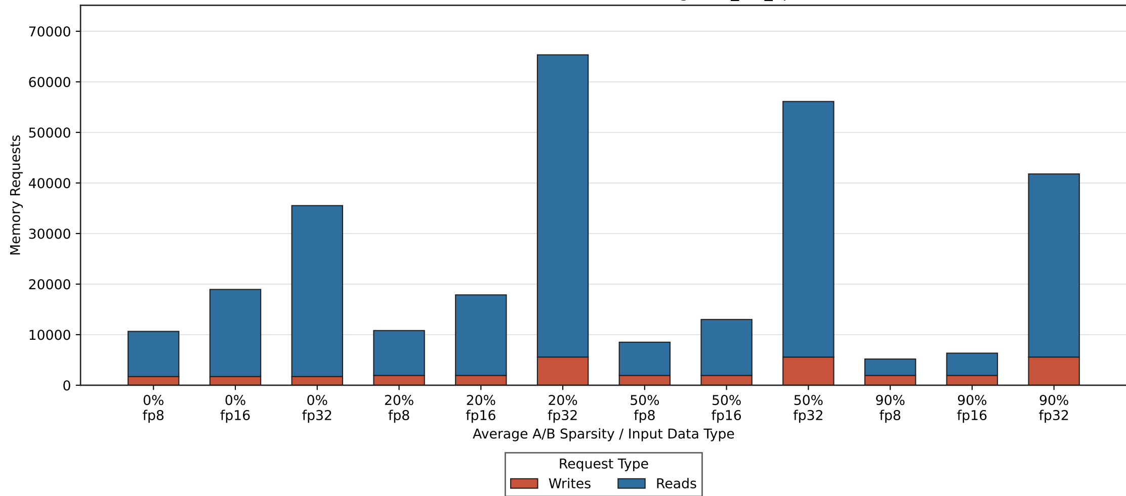
Memory Requests by Sparsity MxNxK=128x128x512, Kernel=sgemm_tcu_op
