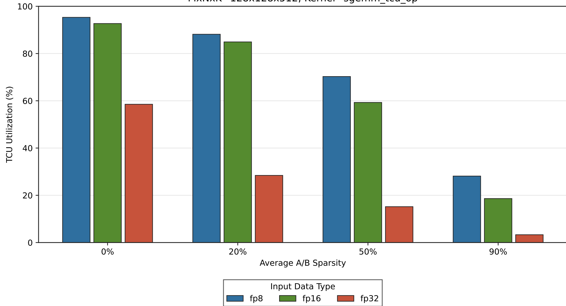
TCU Utilization by OP Sparsity MxNxK=128x128x512, Kernel=sgemm_tcu_op
