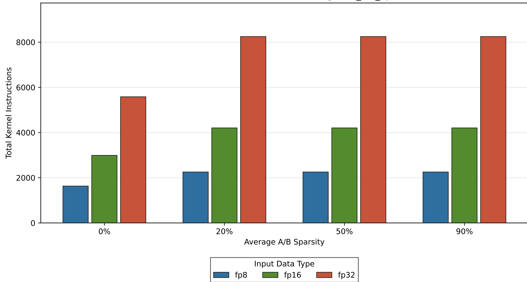
Total Kernel Instructions by OP Sparsity MxNxK=128x128x512, Kernel=sgemmm_tcu_op
