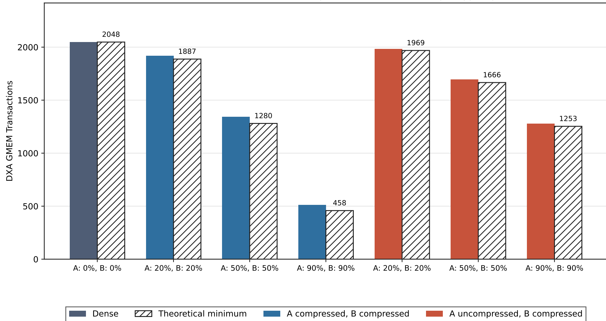
DXA GMEM Transactions - Matrix operation: 64x64x512, Input type: fp8
