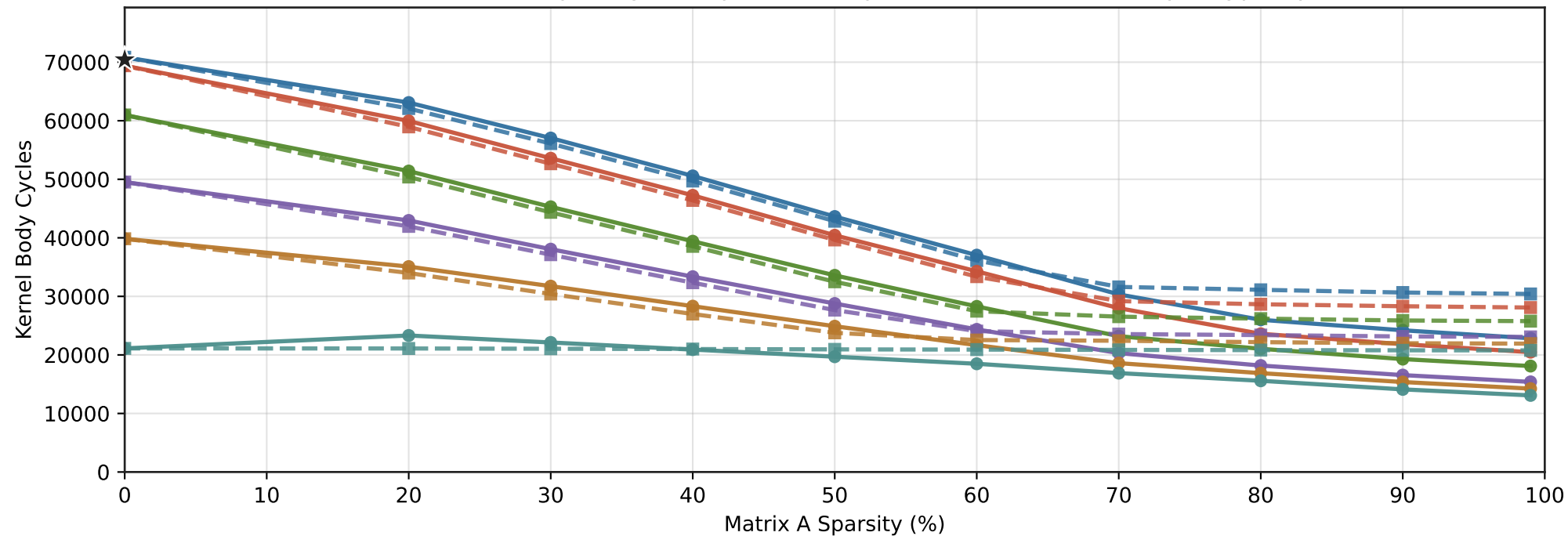
SGEMM TCU OP Sparsity Sweep - Matrix operation: 64x64x512, Input type: fp8
