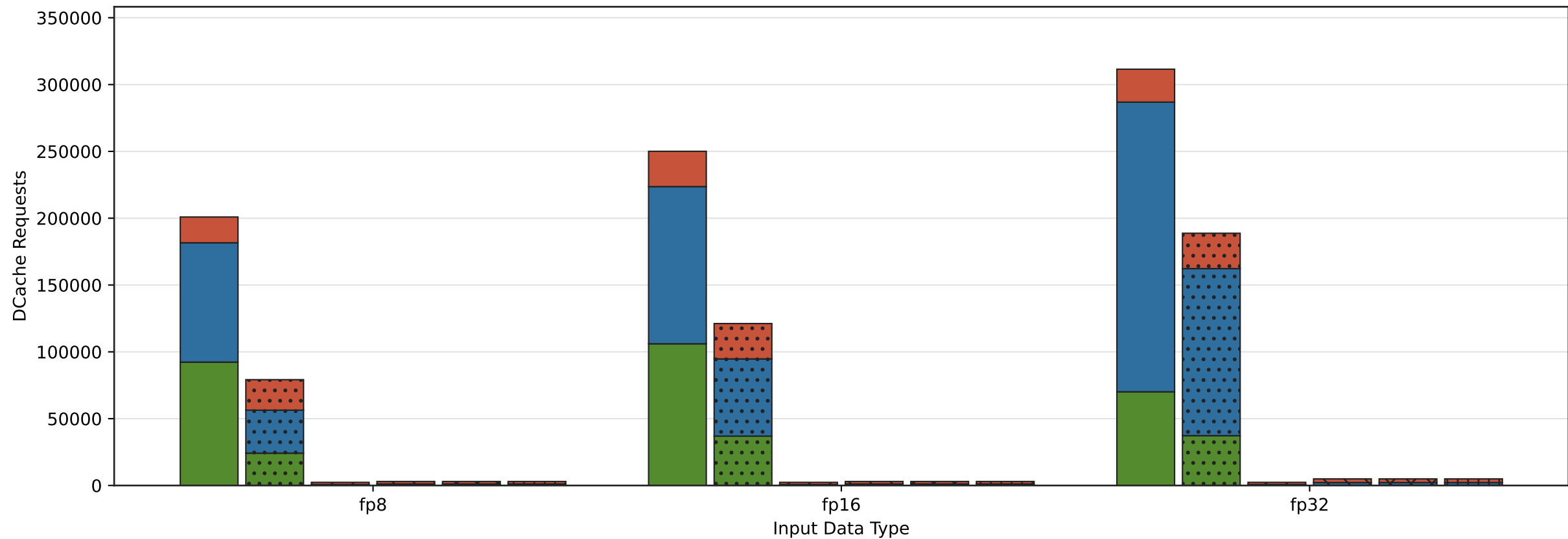
DCache Requests by Input Data Type and Kernel MxNxK=128x128x512
