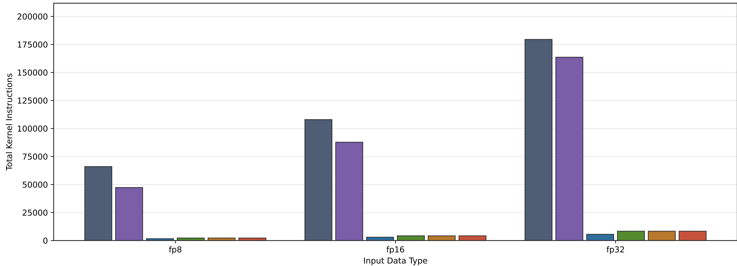
Total Kernel Instructions by Input Data Type MxNxK=128x128x512
