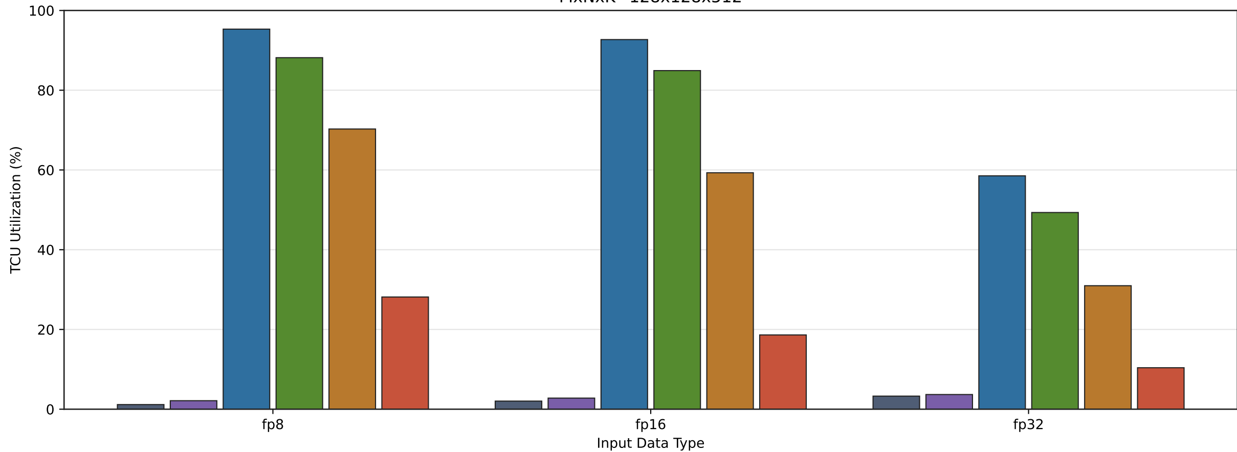
TCU Utilization by Input Data Type MxNxK=128x128x512
