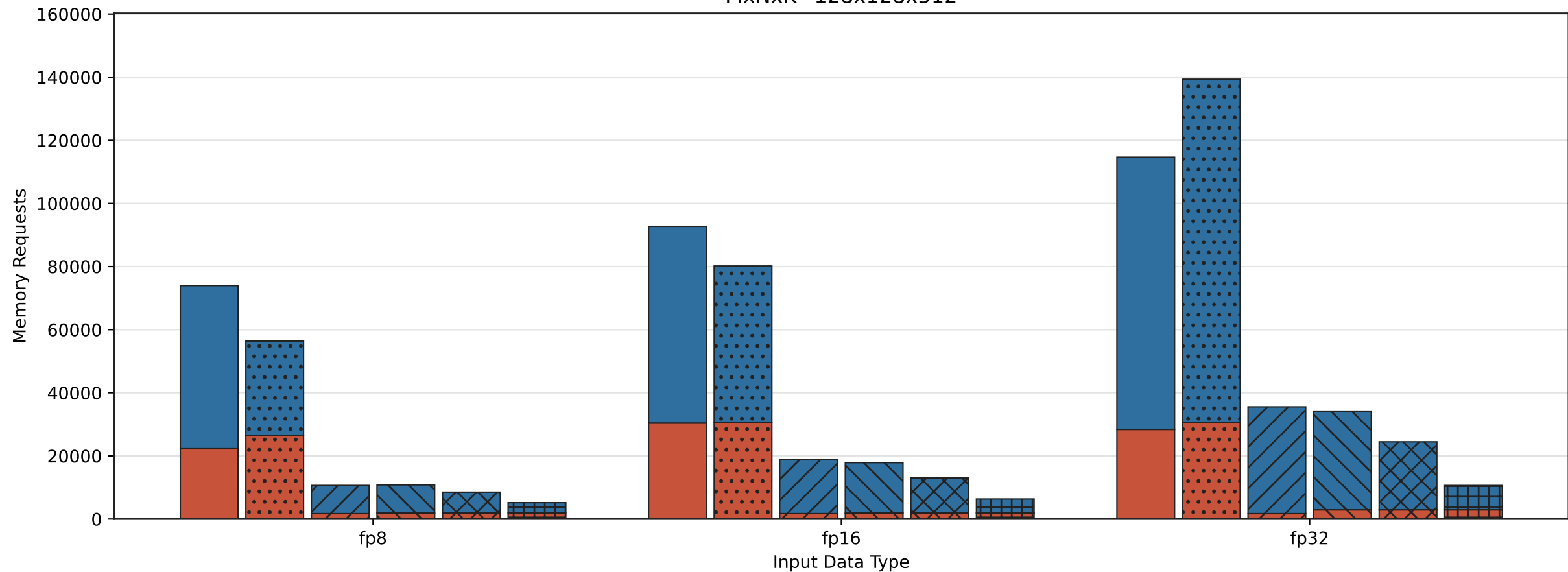
Memory Requests by Input Data Type and Kernel MxNxK=128x128x512
