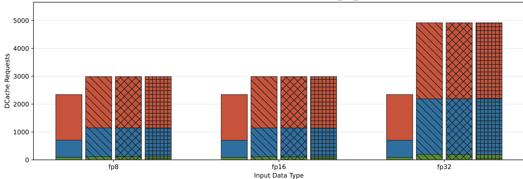
DCache Requests by Input Data Type and OP Sparsity MxNxK=128x128x512, Kernel=sgemmm_tcu_op
