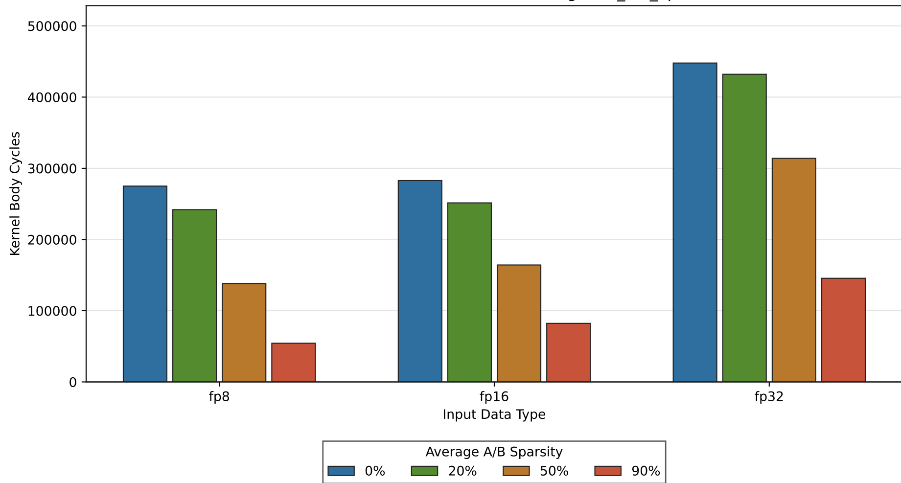
Kernel Body Cycles by Input Data Type and OP Sparsity MxNxK=128x128x512, Kernel=sgemm_tcu_op
