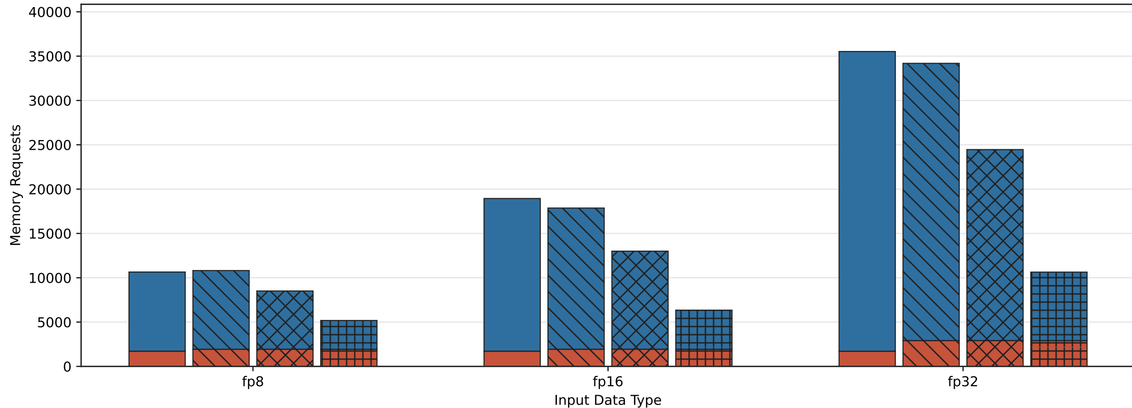
Memory Requests by Input Data Type and OP Sparsity MxNxK=128x128x512, Kernel=sgemm_tcu_op
