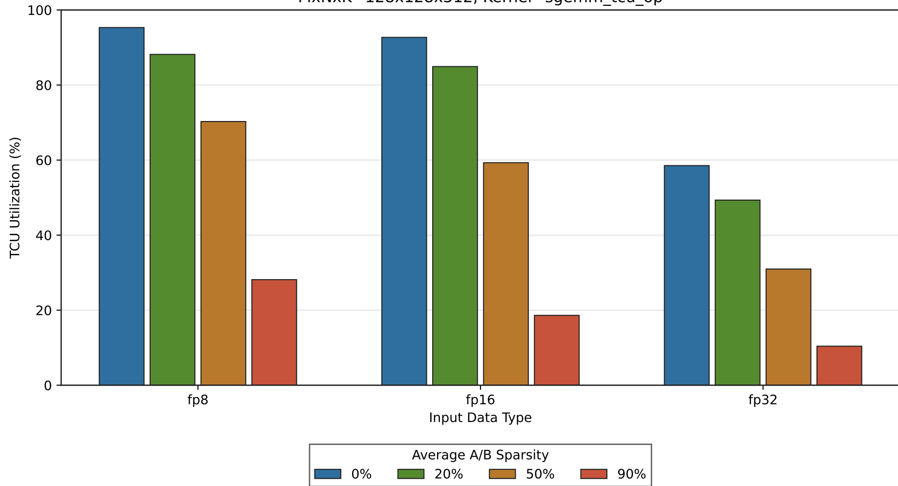
TCU Utilization by Input Data Type and OP Sparsity MxNxK=128x128x512, Kernel=sgemm_tcu_op
