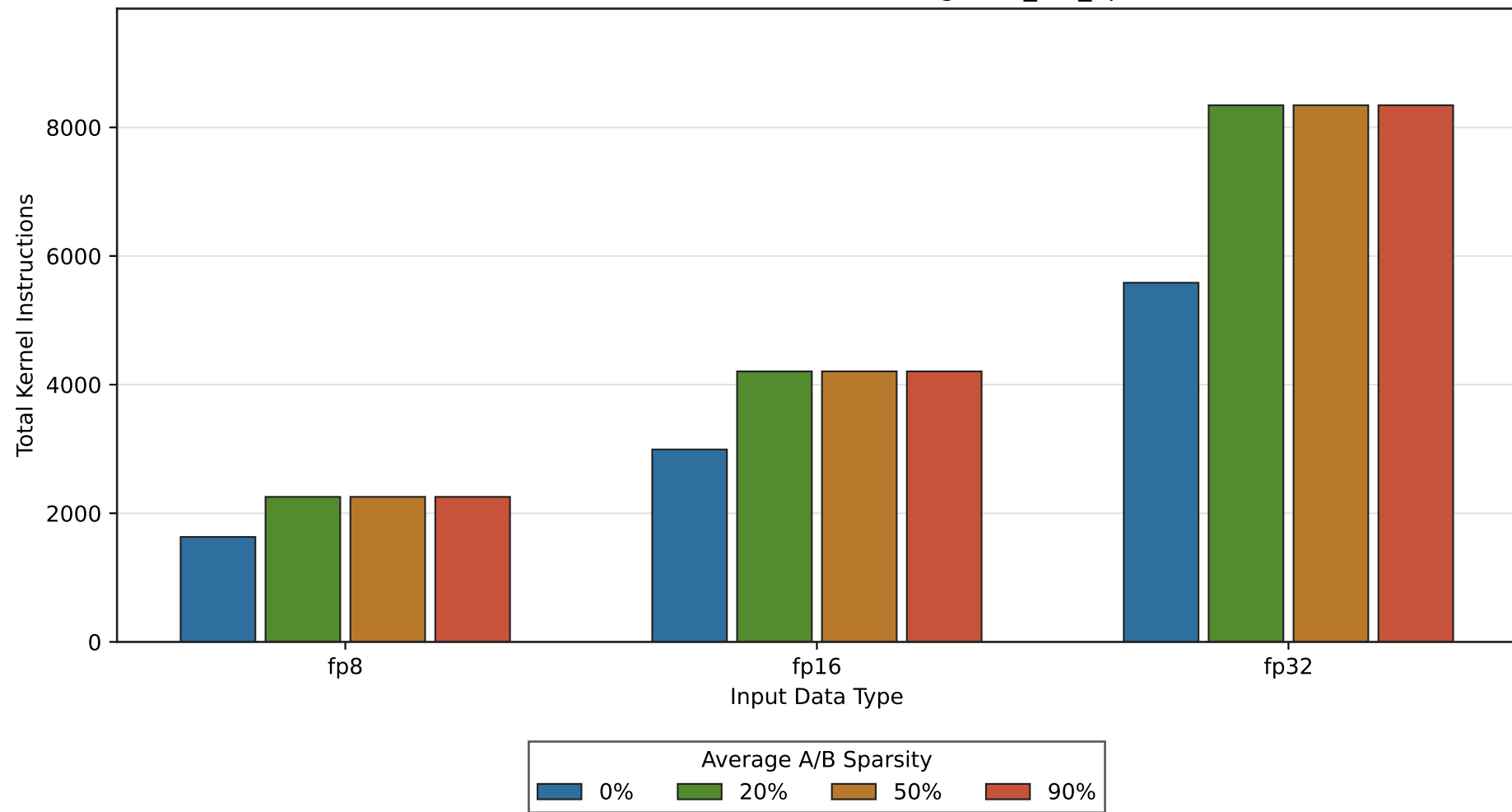
Total Kernel Instructions by Input Data Type and OP Sparsity MxNxK=128x128x512, Kernel=sgemm_tcu_op
