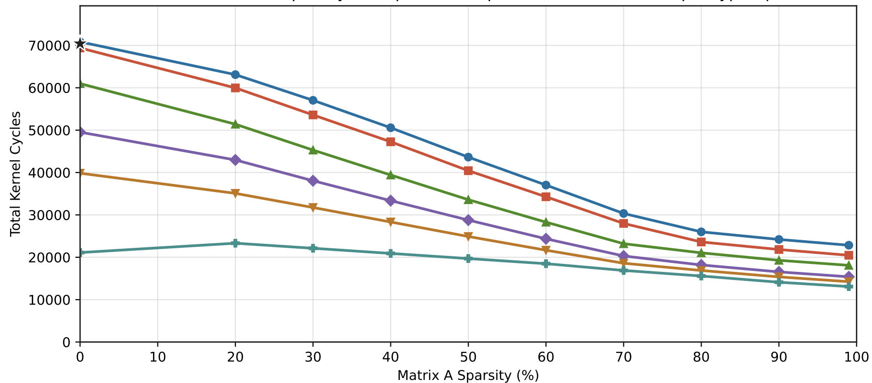
SGEMM TCU OP Sparsity Sweep - Matrix operation: 64x64x512, Input type: fp8
